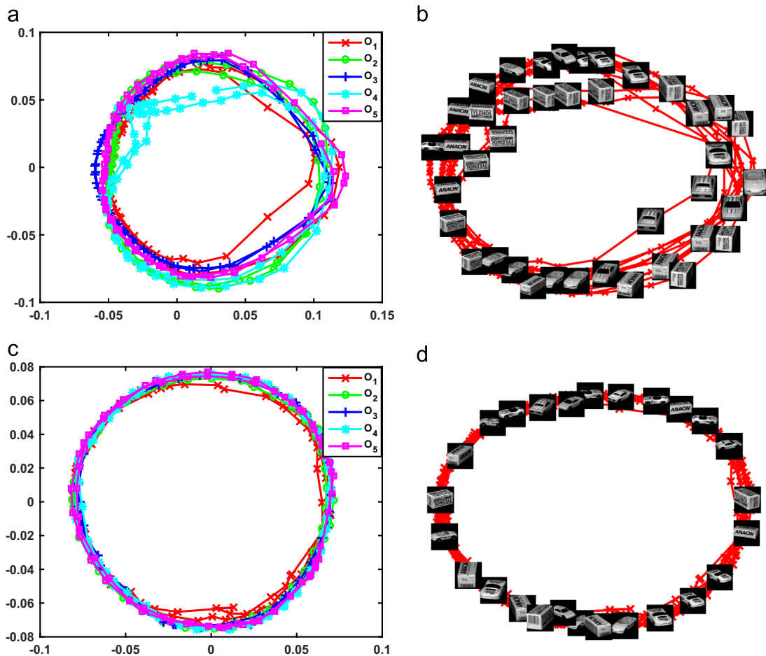
Fig. 10. COIL data set with viewpoint shift: learning a joint view manifold from multiple objects with viewpoint shift. (a) Joint embedding of the view manifold obtained using the proposed algorithm. (b) Joint embedding with random sample images along the manifold. (c) Multiple manifold embedding of the view manifold obtained using the proposed algorithm. (d) Multiple manifold embedding with random sample images along the manifold.
