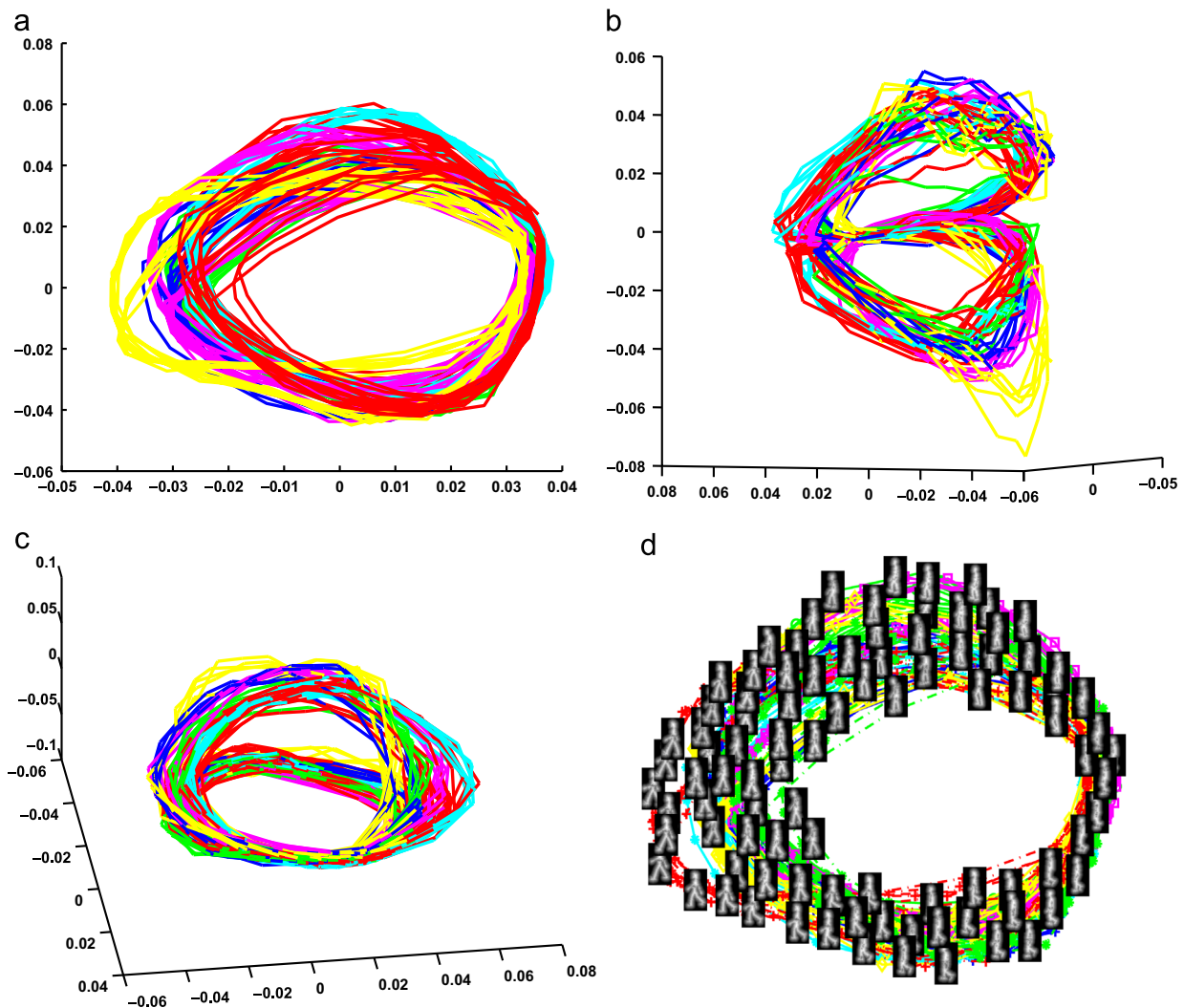
Fig. 11. CMU gait example: embedding the gait manifold from seven subjects. (a), (b), and (c) are different views of the obtained three-dimensional embedding. (d) Visualization with sample images along the manifold. (For interpretation of the references to color in this figure caption, the reader is referred to the web version of this paper.)
