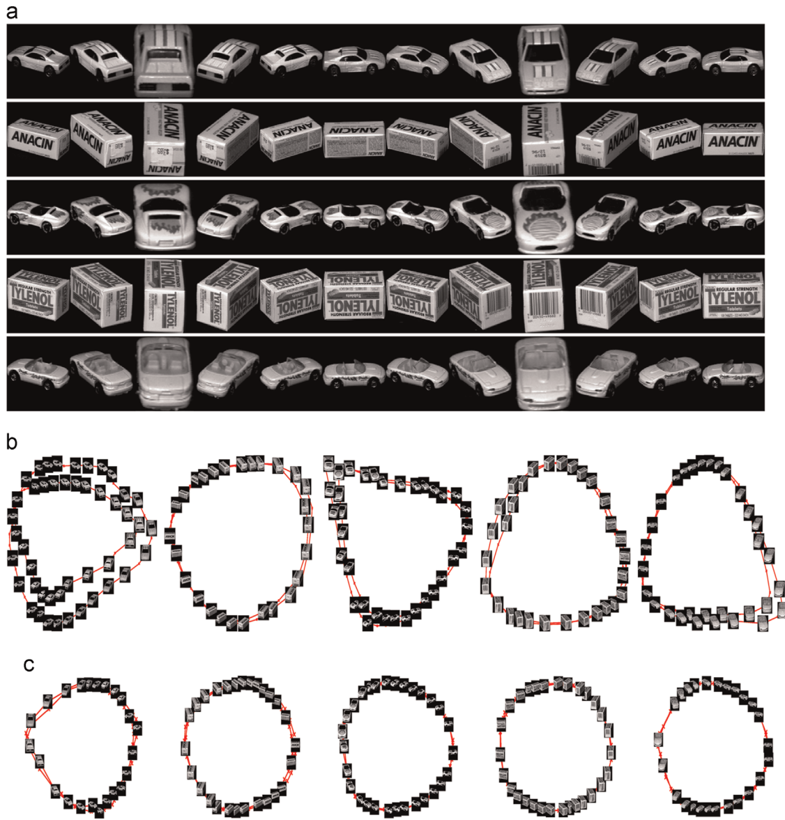
Fig. 4. COIL data set: examples of (a) input object appearance with view variations. (b) Object-specific view manifold embedding using LLE. (c) Object-specific view manifold embedding using Laplacian eigenmap.
