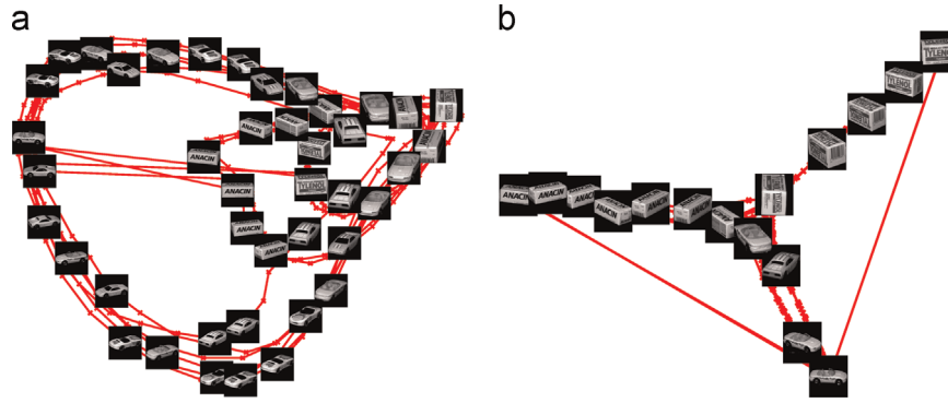
Fig. 5. COIL data set: learning a joint view manifold from multiple objects. (a) LLE embedding for all the data. (b) Laplacian eigenmap embedding of all the data.
