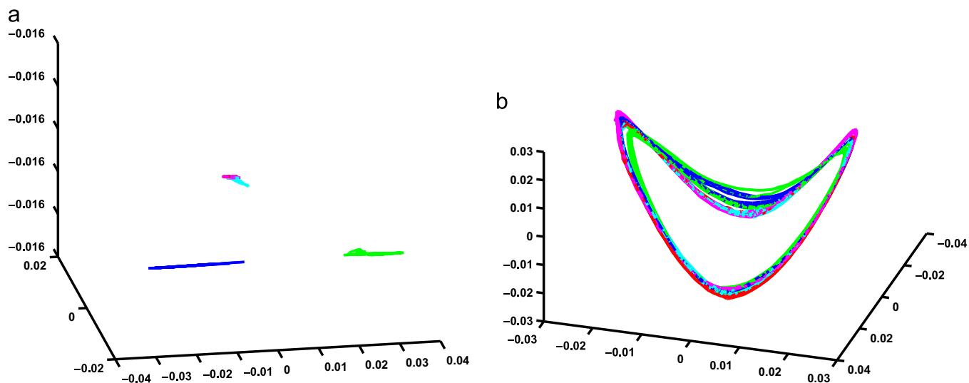
Fig. 13. Learning a kinematic locomotion manifold from different people and different running speeds. (a) Embedding achieved with Laplacian eigenmaps. (b) Joint embedding using the proposed approach. (For interpretation of the references to color in this figure caption, the reader is referred to the web version of this paper.)
