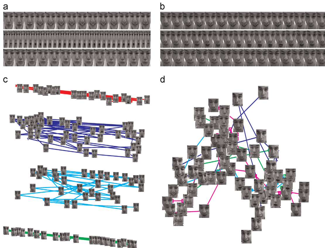
Fig. 12. Embedding of joint facial expressions across different people. (a) and (b) Sample input data for two subjects. (c) Embedding of all the data with Laplacian eigenmaps. Notice the separation between the different people's manifolds. (d) Joint expression embedding obtained by the proposed approach.
