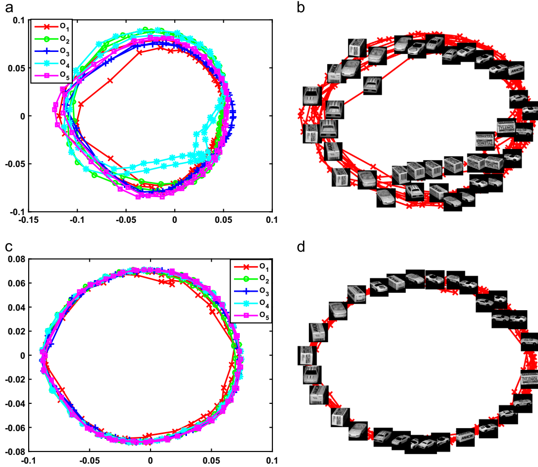
Fig. 7. COIL data set: learning a joint view manifold from multiple objects. (a) Joint embedding of the view manifold obtained using the proposed algorithm. (b) Joint embedding with random sample images along the manifold. (c) Multiple manifold embedding of the view manifold obtained using [39]. (d) Multiple manifold embedding with random sample images along the manifold. (For interpretation of the references to color in this figure caption, the reader is referred to the web version of this paper.)
