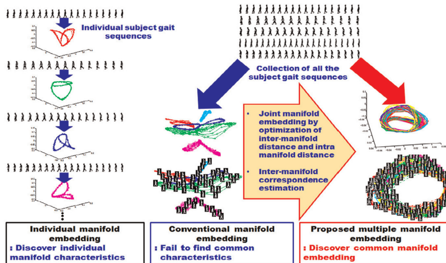
Fig. 3. Diagram to compare conventional manifold embedding for individual data sets and collection of data sets with the proposed joint manifold embedding.
