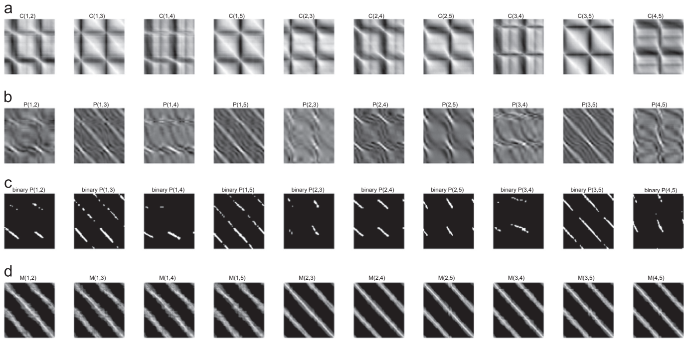
Fig. 9. COIL data set with viewpoint shift: learning a joint view manifold from multiple objects without implicit alignment. (a) Pairwise correspondence matrices ( C_{shift}^{1,2}, C_{shift}^{1,3}, C_{shift}^{1,4}, C_{shift}^{1,5}, C_{shift}^{2,3}, C_{shift}^{2,4}, C_{shift}^{2,5}, C_{shift}^{3,4}, C_{shift}^{3,5}, C_{shift}^{4,5} ). (b) Pairwise permutation matrices ( p_{shift}^{1,2}, p_{shift}^{1,3}, p_{shift}^{1,4}, p_{shift}^{1,5}, p_{shift}^{2,3}, p_{shift}^{2,4}, p_{shift}^{2,5}, p_{shift}^{3,4}, p_{shift}^{3,5}, p_{shift}^{4,5} ). (c) Binalization of pairwise permutation matrices. (d) Pairwise soft correspondence matrices ( M_{shift}^{1,2}, M_{shift}^{1,3}, M_{shift}^{1,4}, M_{shift}^{1,5}, M_{shift}^{2,3}, M_{shift}^{2,4}, M_{shift}^{2,5}, M_{shift}^{3,4}, M_{shift}^{3,5}, M_{shift}^{4,5} ).
