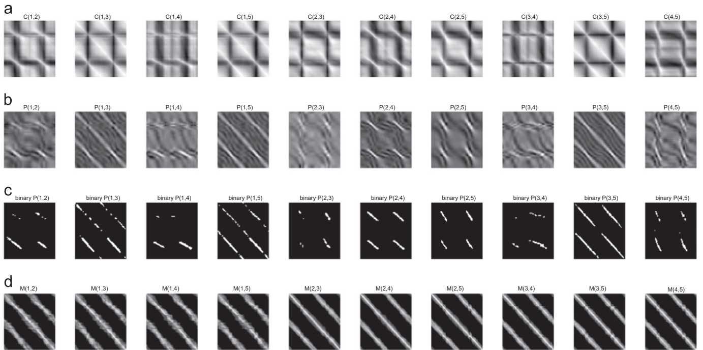
Fig. 6. COIL data set: learning a joint view manifold from multiple objects. (a) Pairwise correspondence matrices ( C^{1,2}, C^{1,3}, C^{1,4}, C^{1,5}, C^{2,3}, C^{2,4}, C^{2,5}, C^{3,4}, C^{3,5}, C^{4,5} ). (b) Pairwise permutation matrices ( p^{1,2}, p^{1,3}, p^{1,4}, p^{1,5}, p^{2,3}, p^{2,4}, p^{2,5}, p^{3,4}, p^{3,5}, p^{4,5} ). (c) Binarization of pairwise permutation matrices. (d) Pairwise soft correspondence matrices ( M^{1,2}, M^{1,3}, M^{1,4}, M^{1,5}, M^{2,3}, M^{2,4}, M^{2,5}, M^{3,4}, M^{3,5}, M^{4,5} ) [39].
